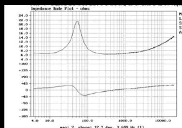
Impedance & Phase
